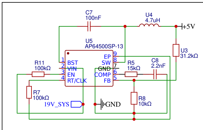
PWR Delivery - 5V
